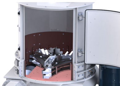
A Large maintenance door for optimal accessibility
